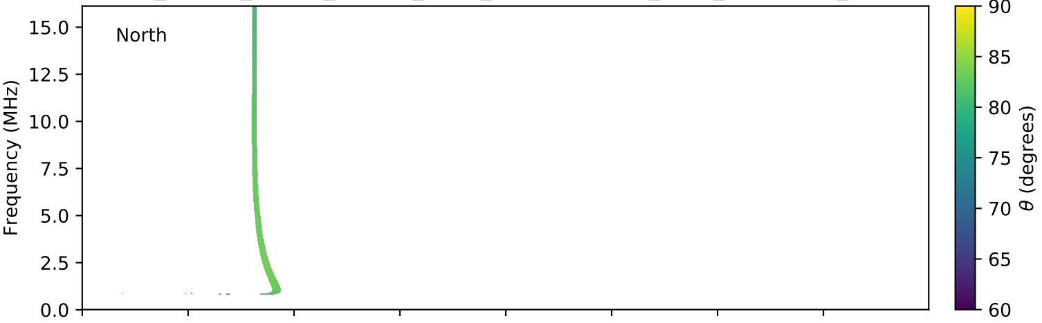
expres_cassini_jupiter_europa_isaac_lossc-wid1deg_3kev_20001219_v01.cdf
