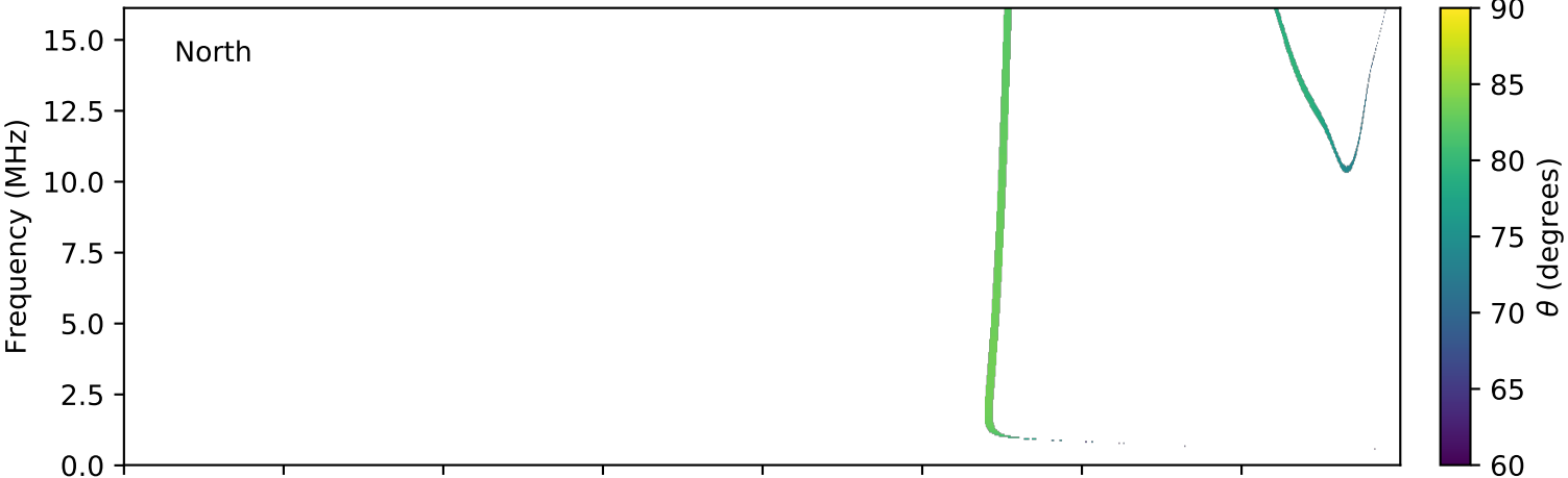
expres_cassini_jupiter_europa_isaac_lossc-wid1deg_3kev_20001217_v01.cdf
