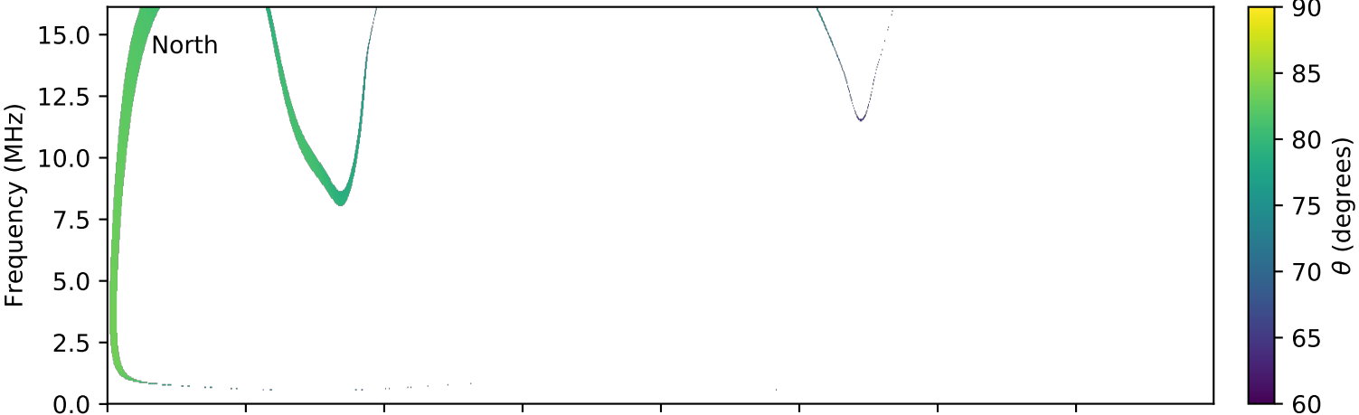
expres_cassini_jupiter_europa_isaac_lossc-wid1deg_3kev_20001214_v01.cdf
