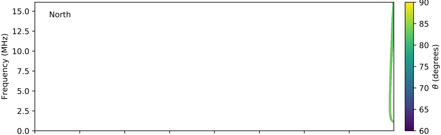
expres_cassini_jupiter_europa_isaac_lossc-wid1deg_3kev_20001213_v01.cdf
