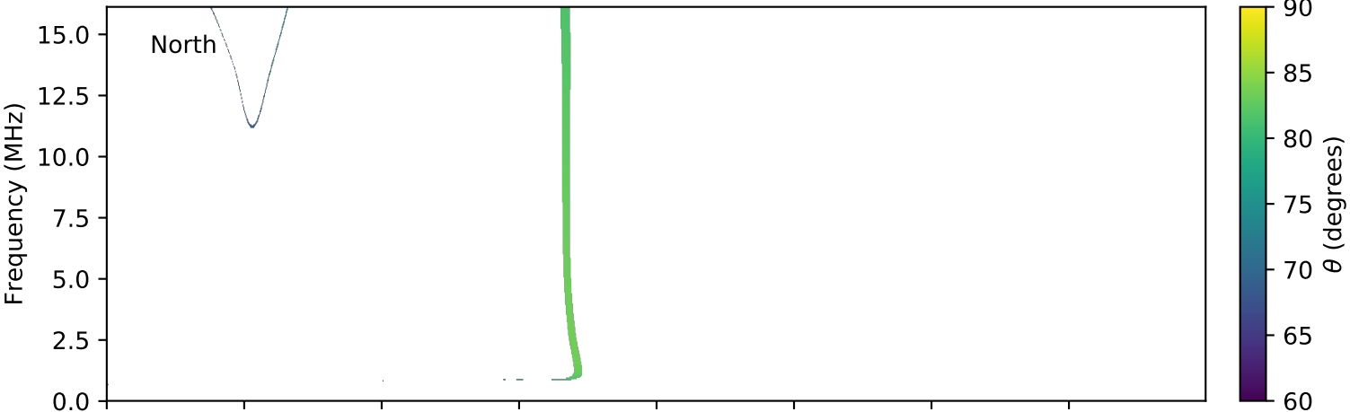
expres_cassini_jupiter_europa_isaac_lossc-wid1deg_3kev_20001208_v01.cdf
