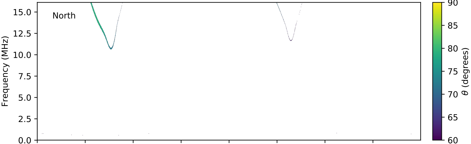
expres_cassini_jupiter_europa_isaac_lossc-wid1deg_3kev_20001207_v01.cdf
