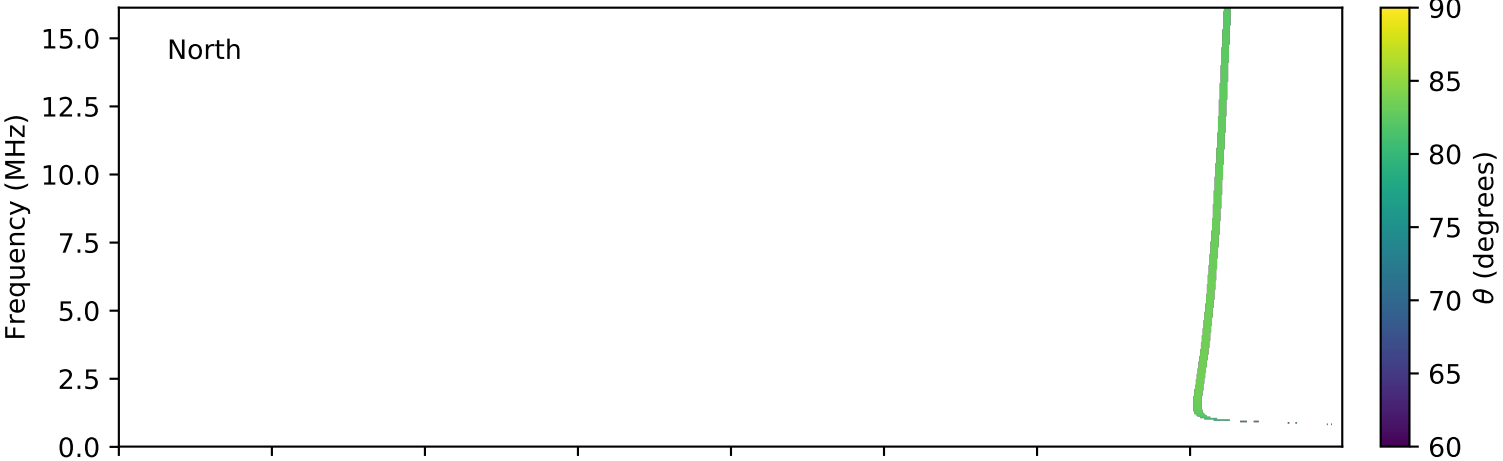
expres_cassini_jupiter_europa_isaac_lossc-wid1deg_3kev_20001206_v01.cdf
