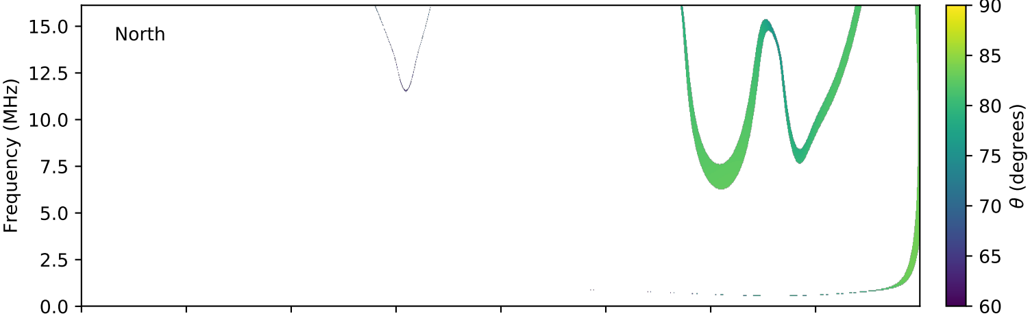
expres_cassini_jupiter_europa_isaac_lossc-wid1deg_3kev_20001204_v01.cdf
