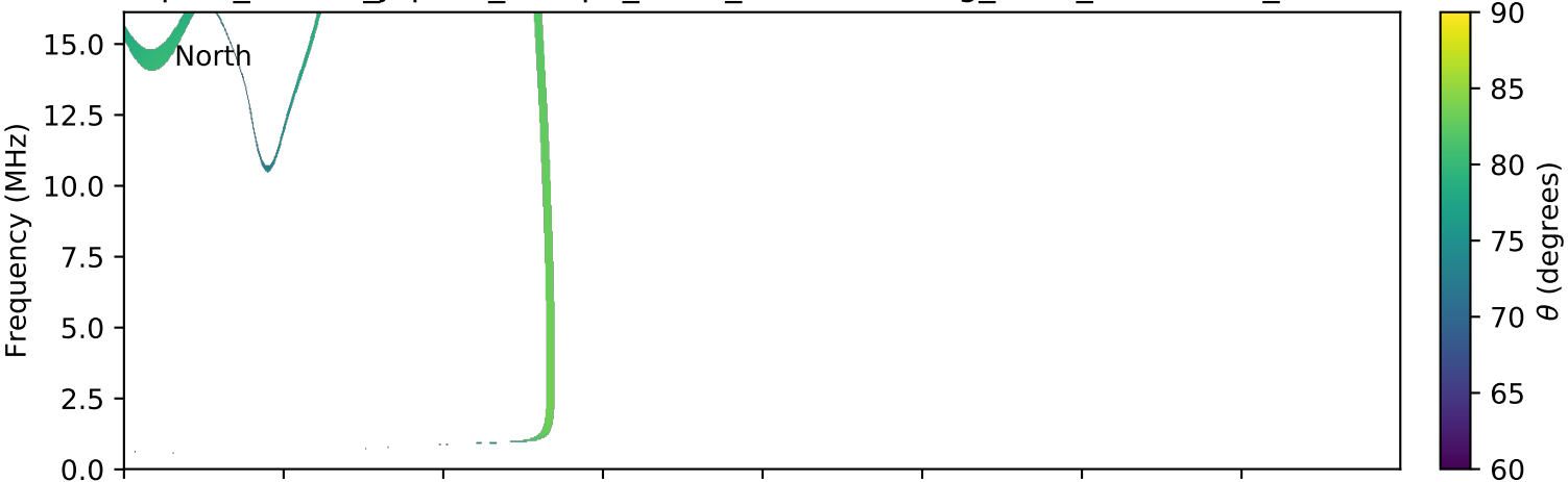
expres_cassini_jupiter_europa_isaac_lossc-wid1deg_3kev_20001201_v01.cdf
