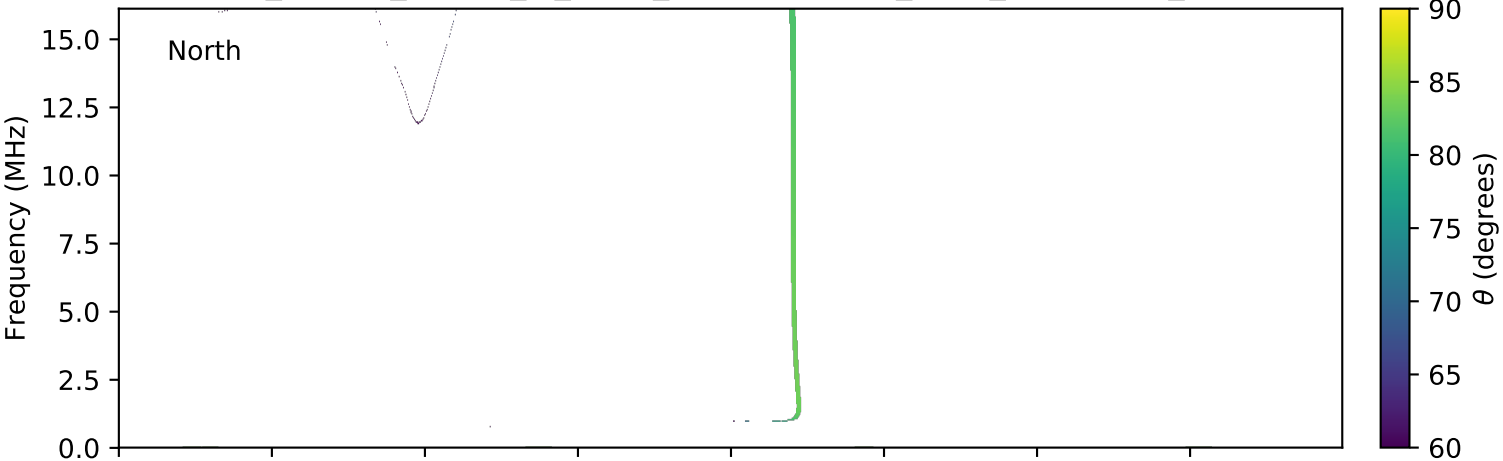
expres_cassini_jupiter_io_isaac_lossc-wid1deg_3kev_20001130_v01.cdf
