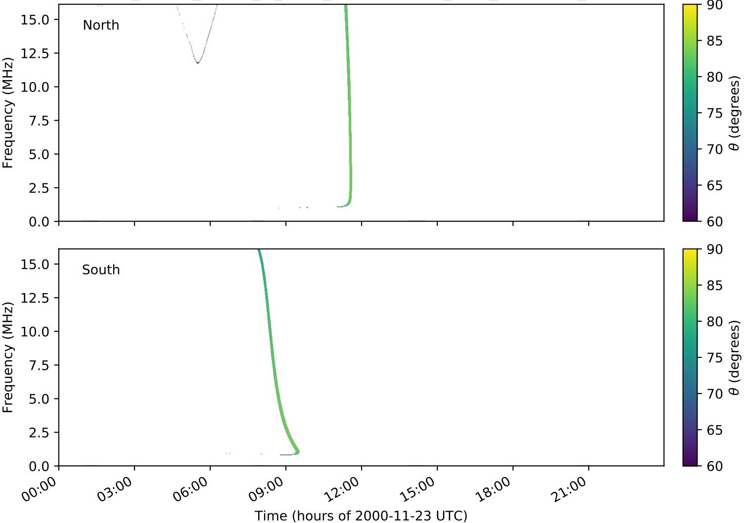
expres_cassini_jupiter_io_isaac_lossc-wid1deg_3kev_20001123_v01.cdf
