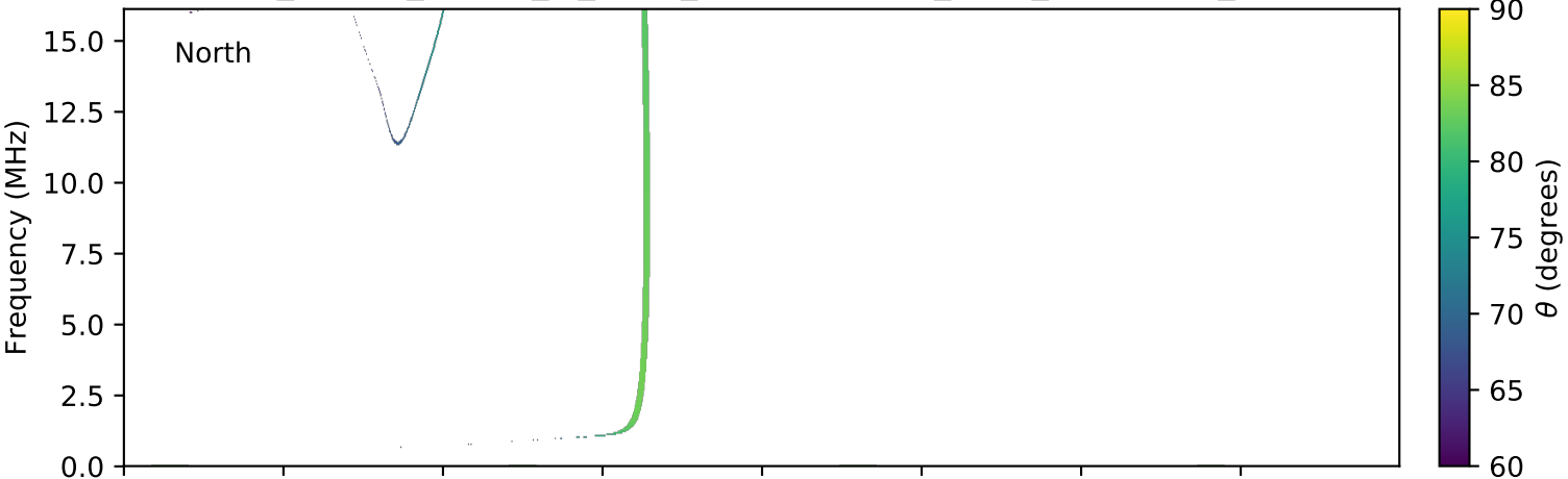
expres_cassini_jupiter_io_isaac_lossc-wid1deg_3kev_20001116_v01.cdf
