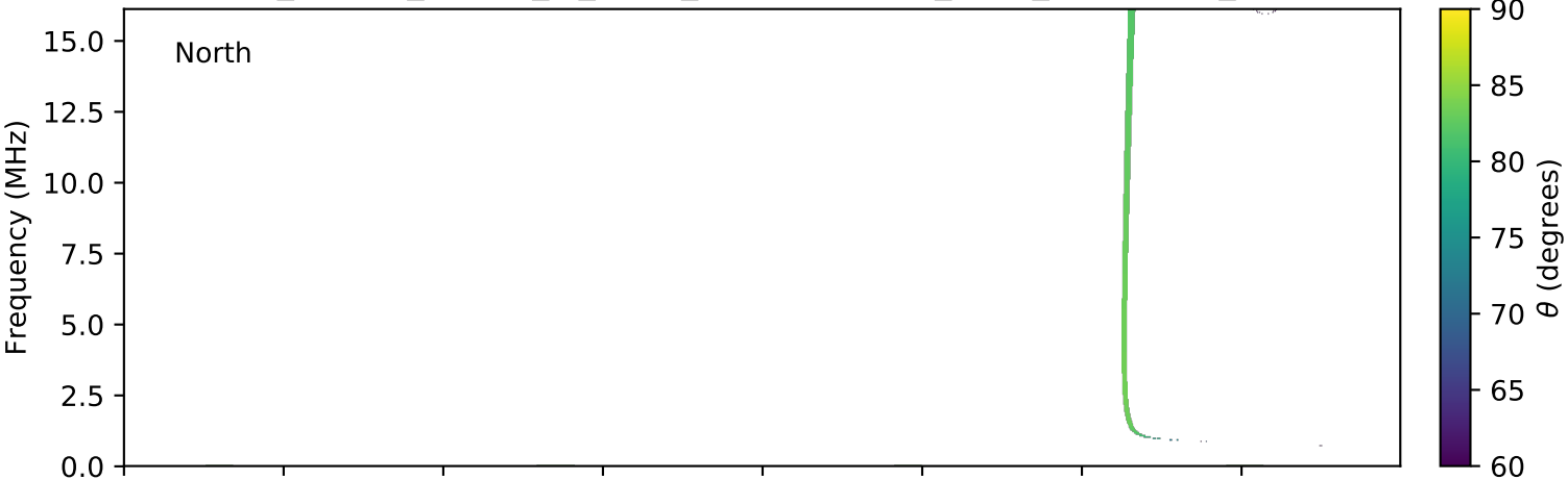
expres_cassini_jupiter_io_isaac_lossc-wid1deg_3kev_20001113_v01.cdf
