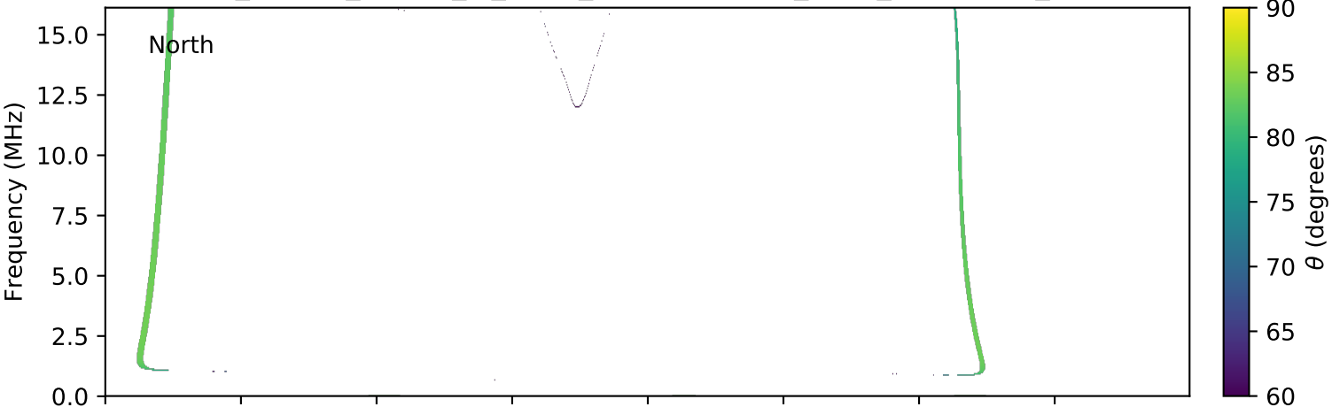
expres_cassini_jupiter_io_isaac_lossc-wid1deg_3kev_20001112_v01.cdf
