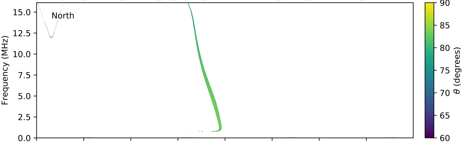
expres_cassini_jupiter_io_isaac_lossc-wid1deg_3kev_20001107_v01.cdf
