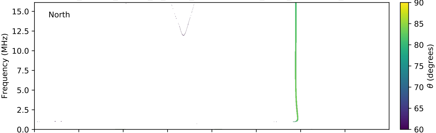
expres_cassini_jupiter_io_isaac_lossc-wid1deg_3kev_20001105_v01.cdf
