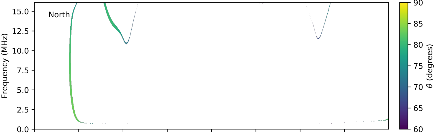
expres_cassini_jupiter_io_isaac_lossc-wid1deg_3kev_20001103_v01.cdf
