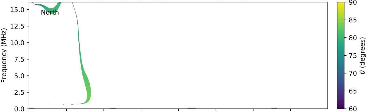
expres_cassini_jupiter_io_isaac_lossc-wid1deg_3kev_20001102_v01.cdf
