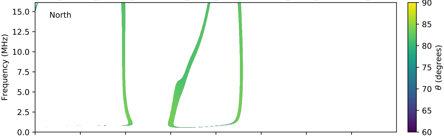
expres_cassini_jupiter_ganymede_isaac_lossc-wid1deg_3kev_20001127_v01.cdf
