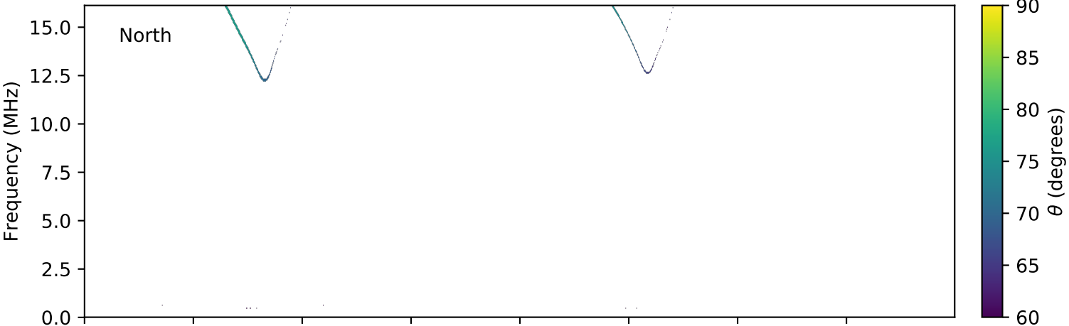
expres_cassini_jupiter_ganymede_isaac_lossc-wid1deg_3kev_20001125_v01.cdf
