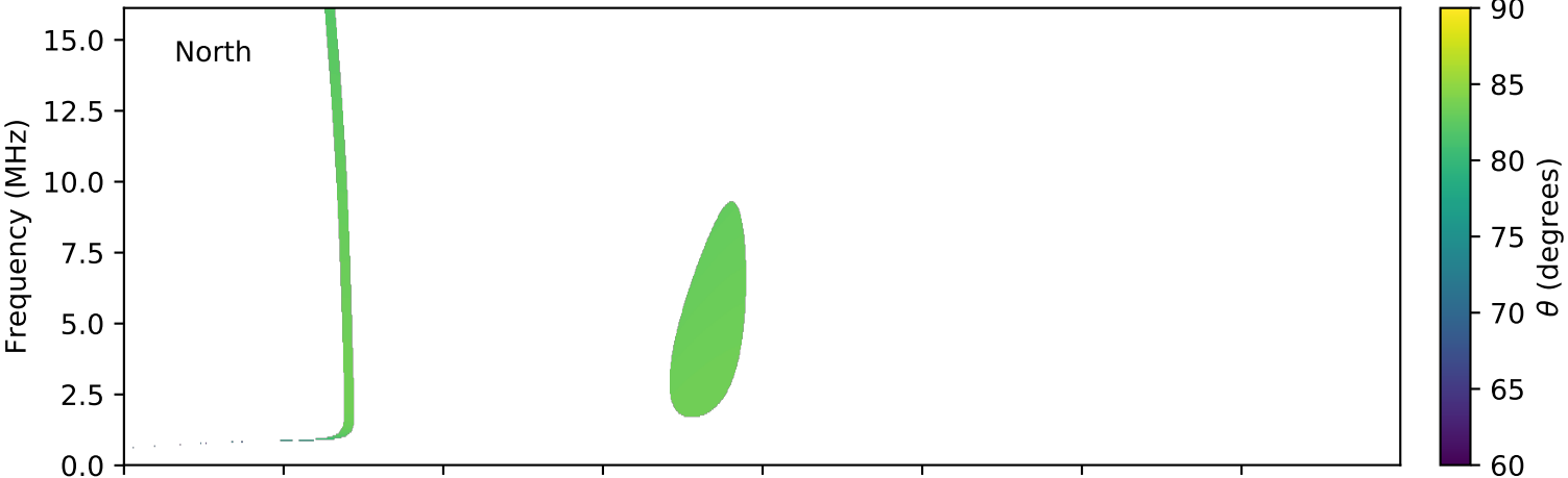
expres_cassini_jupiter_ganymede_isaac_lossc-wid1deg_3kev_20001120_v01.cdf
