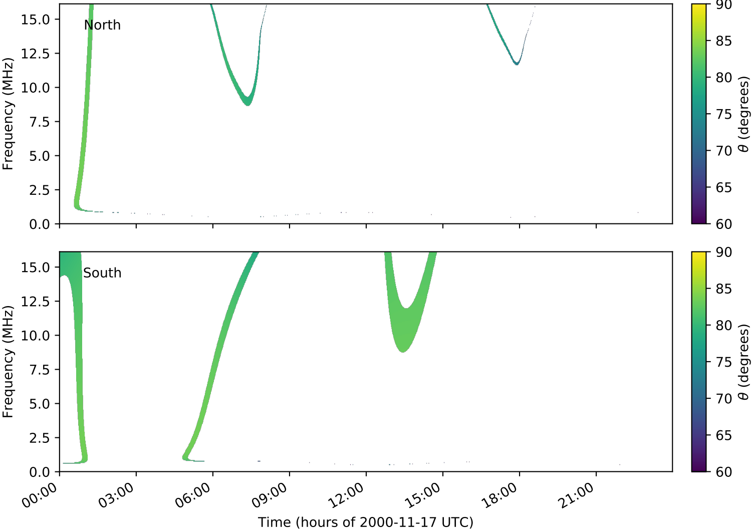
expres_cassini_jupiter_ganymede_isaac_lossc-wid1deg_3kev_20001117_v01.cdf
