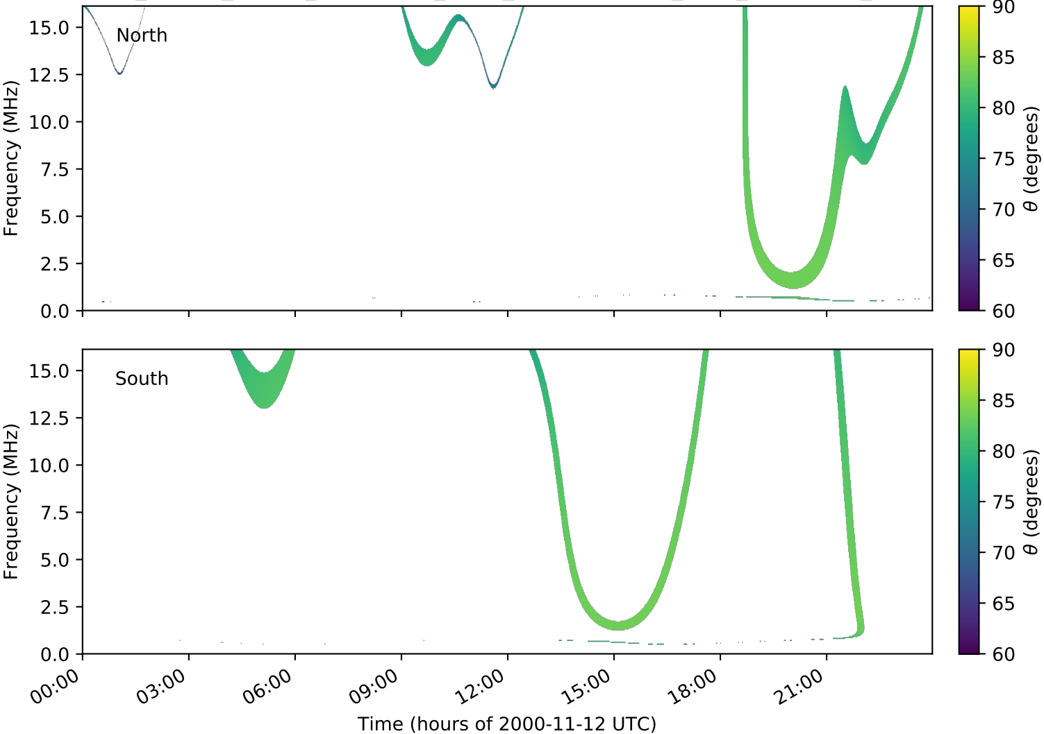
expres_cassini_jupiter_ganymede_isaac_lossc-wid1deg_3kev_20001112_v01.cdf
