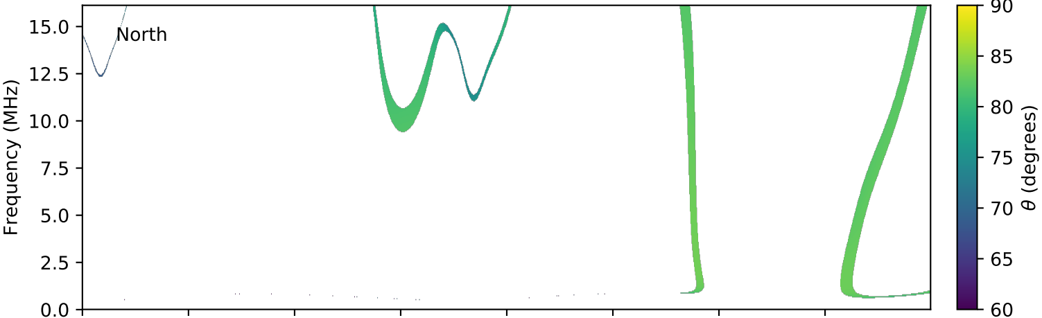
expres_cassini_jupiter_ganymede_isaac_lossc-wid1deg_3kev_20001105_v01.cdf
