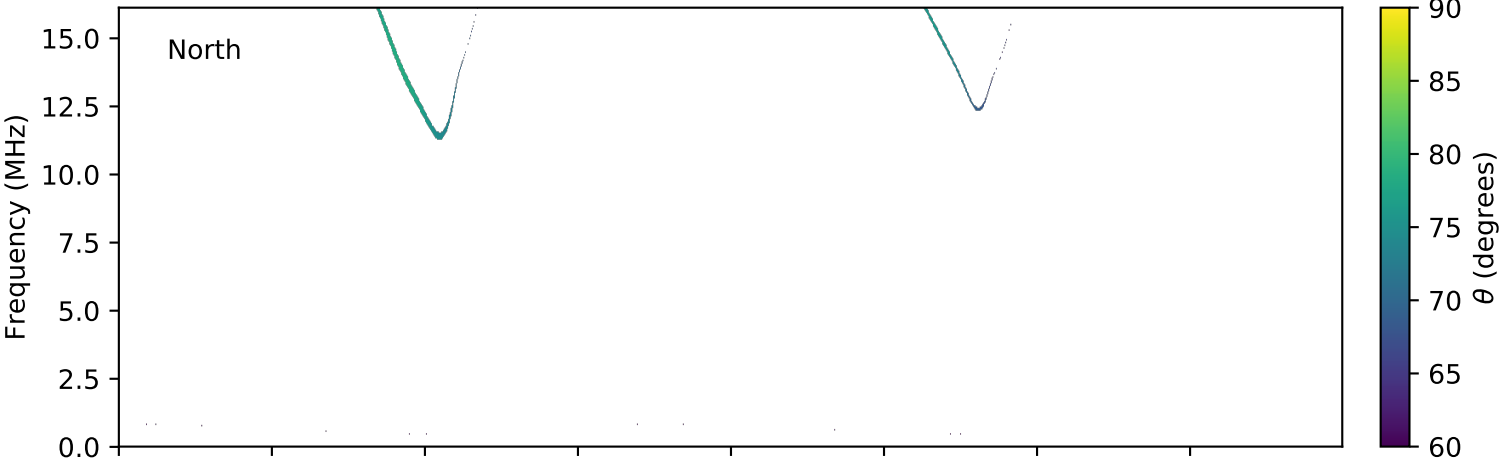
expres_cassini_jupiter_ganymede_isaac_lossc-wid1deg_3kev_20001103_v01.cdf
