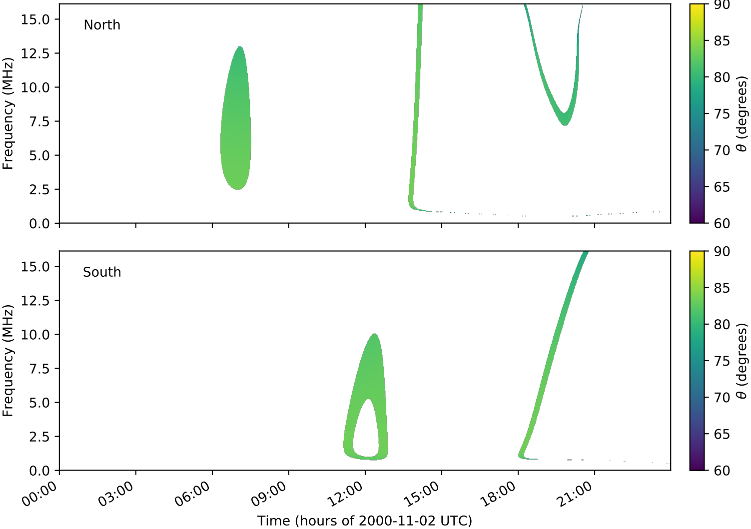
expres_cassini_jupiter_ganymede_isaac_lossc-wid1deg_3kev_20001102_v01.cdf
