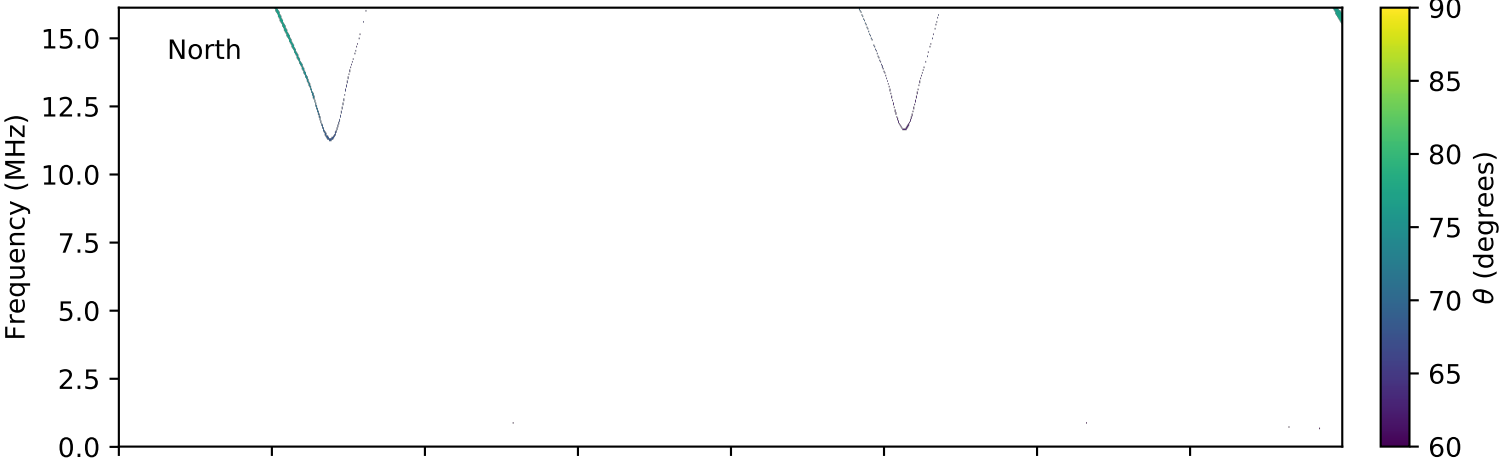
expres_cassini_jupiter_europa_isaac_lossc-wid1deg_3kev_20001130_v01.cdf
