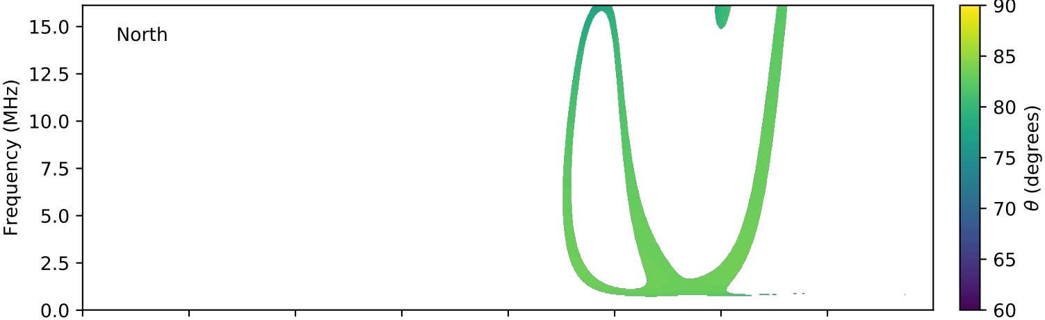
expres_cassini_jupiter_europa_isaac_lossc-wid1deg_3kev_20001129_v01.cdf
