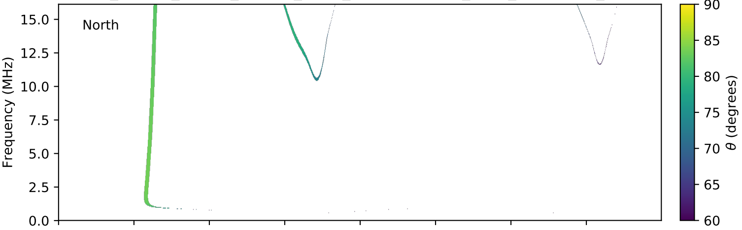
expres_cassini_jupiter_europa_isaac_lossc-wid1deg_3kev_20001126_v01.cdf
