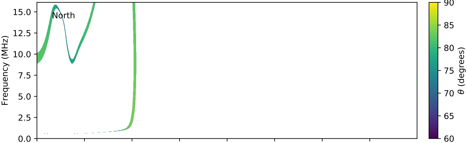
expres_cassini_jupiter_europa_isaac_lossc-wid1deg_3kev_20001124_v01.cdf
