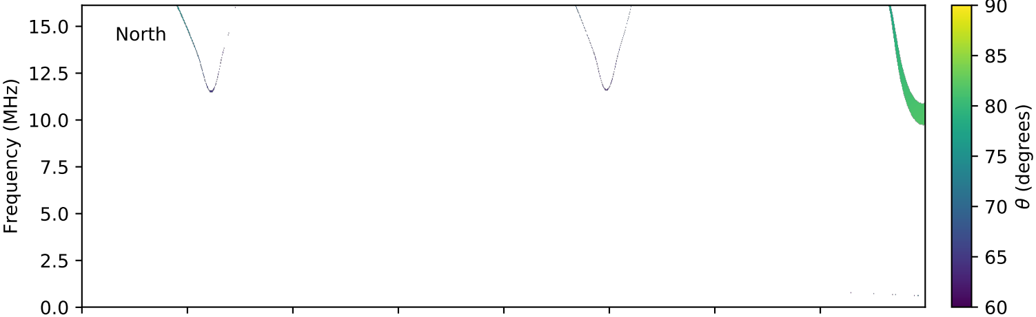
expres_cassini_jupiter_europa_isaac_lossc-wid1deg_3kev_20001123_v01.cdf
