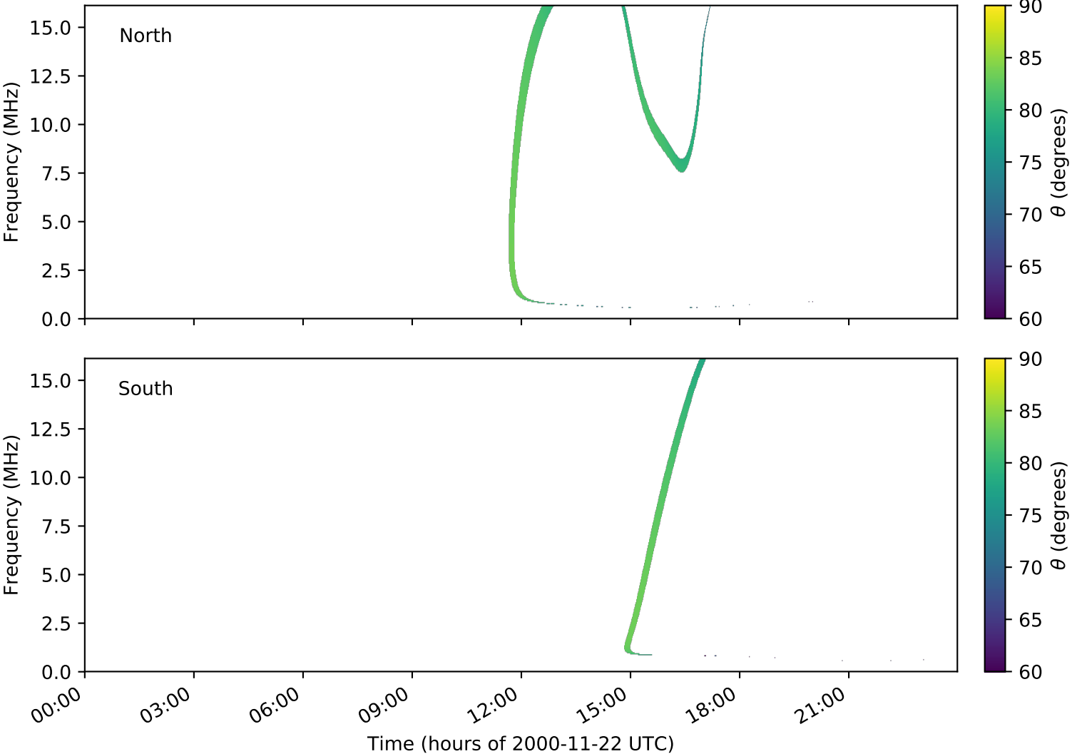
expres_cassini_jupiter_europa_isaac_lossc-wid1deg_3kev_20001122_v01.cdf
