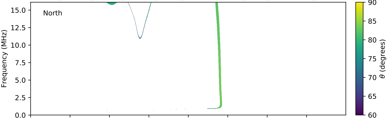
expres_cassini_jupiter_europa_isaac_lossc-wid1deg_3kev_20001120_v01.cdf
