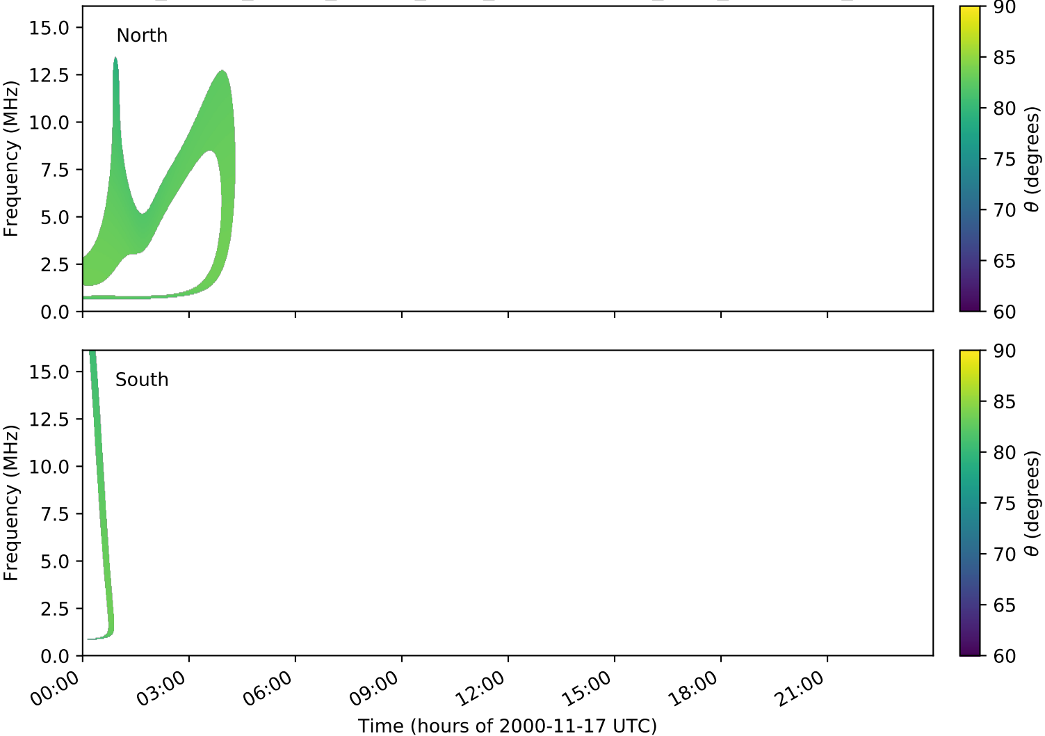
expres_cassini_jupiter_europa_isaac_lossc-wid1deg_3kev_20001117_v01.cdf
