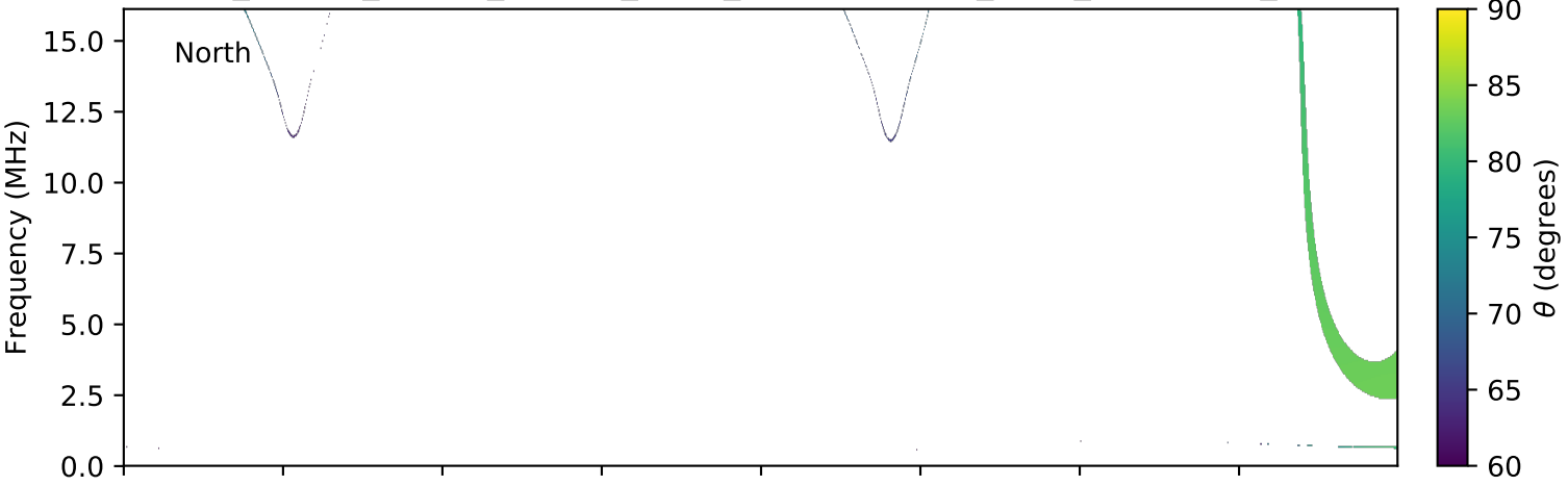
expres_cassini_jupiter_europa_isaac_lossc-wid1deg_3kev_20001116_v01.cdf
