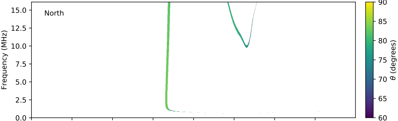
expres_cassini_jupiter_europa_isaac_lossc-wid1deg_3kev_20001115_v01.cdf
