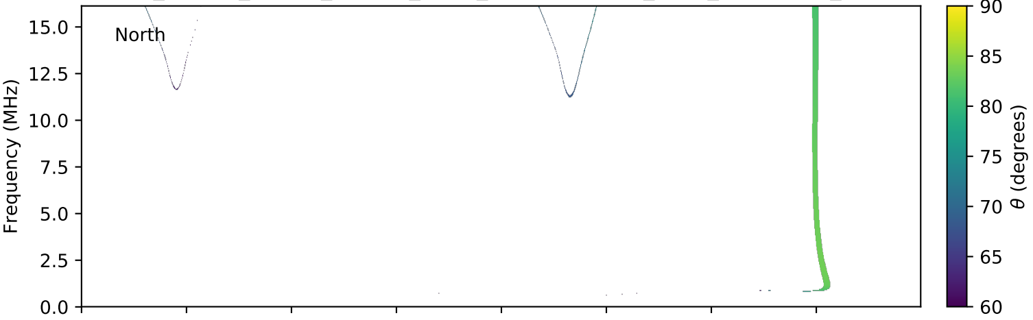
expres_cassini_jupiter_europa_isaac_lossc-wid1deg_3kev_20001109_v01.cdf
