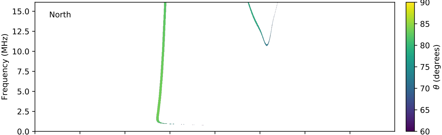
expres_cassini_jupiter_europa_isaac_lossc-wid1deg_3kev_20001108_v01.cdf
