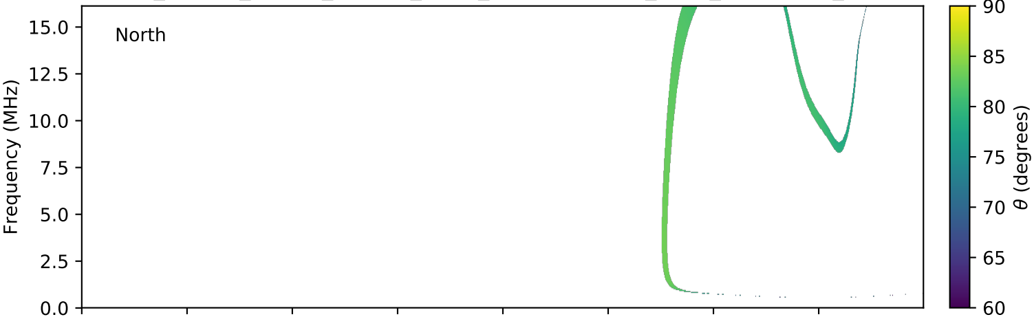
expres_cassini_jupiter_europa_isaac_lossc-wid1deg_3kev_20001104_v01.cdf
