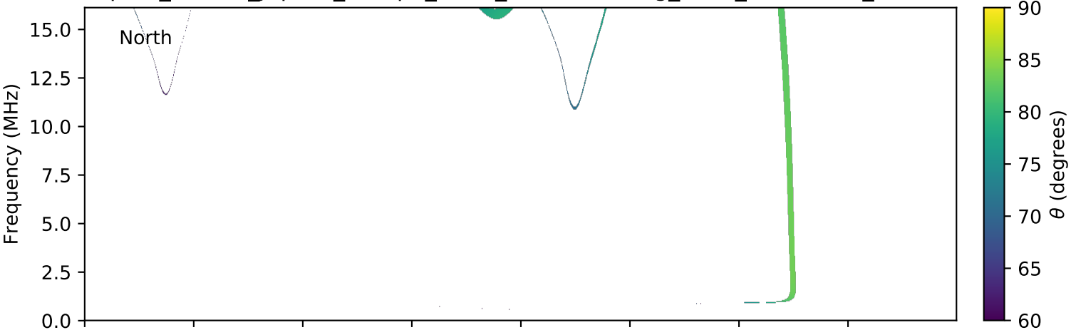
expres_cassini_jupiter_europa_isaac_lossc-wid1deg_3kev_20001102_v01.cdf
