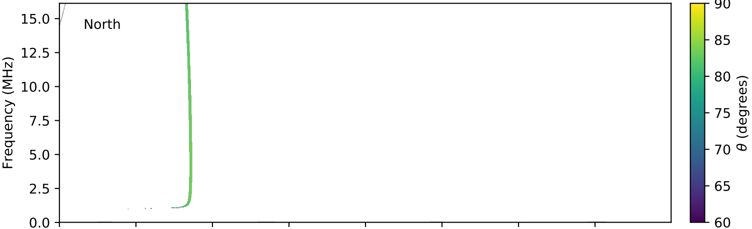
expres_cassini_jupiter_io_isaac_lossc-wid1deg_3kev_20001010_v01.cdf
