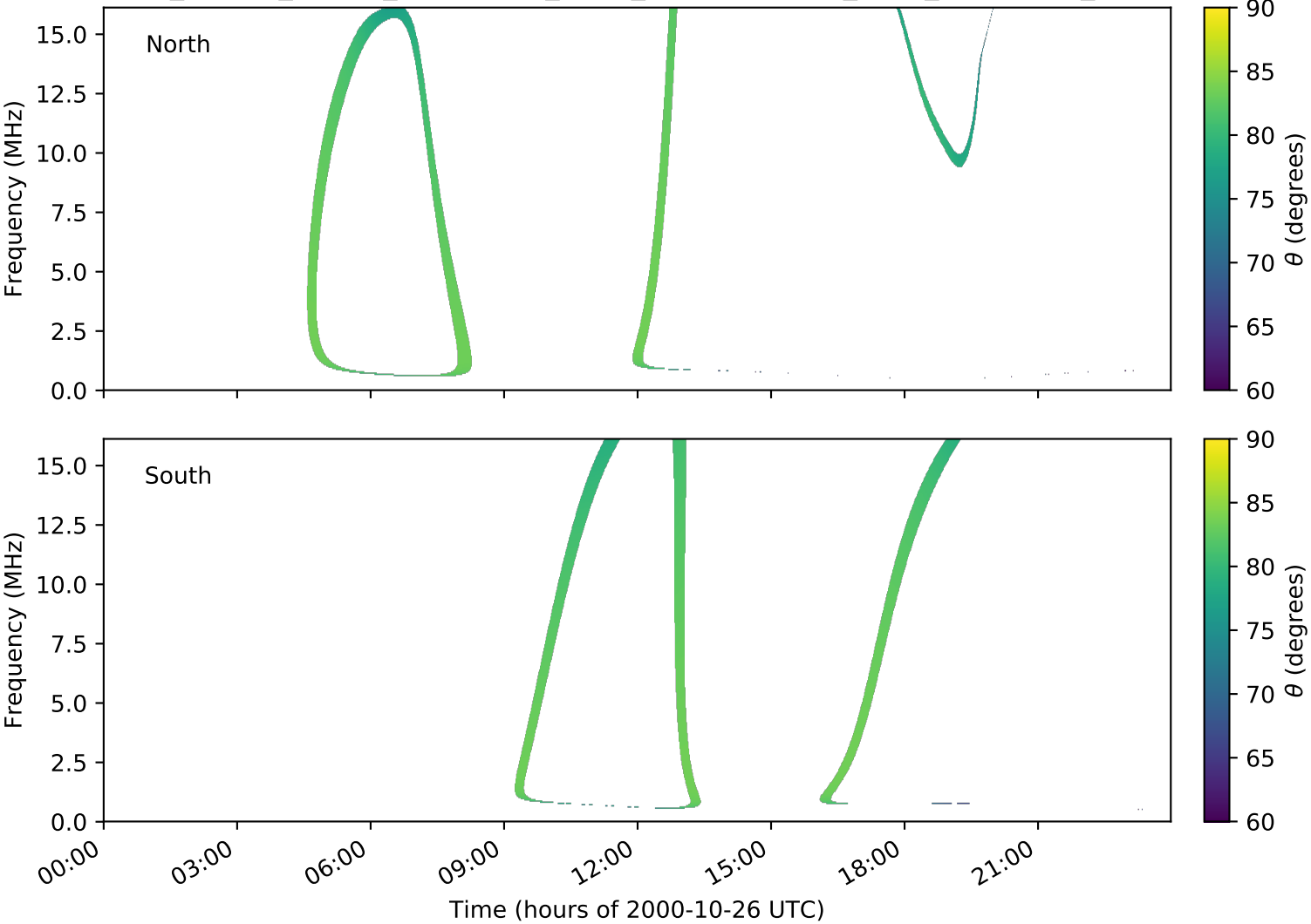
expres_cassini_jupiter_ganymede_isaac_lossc-wid1deg_3kev_20001026_v01.cdf
