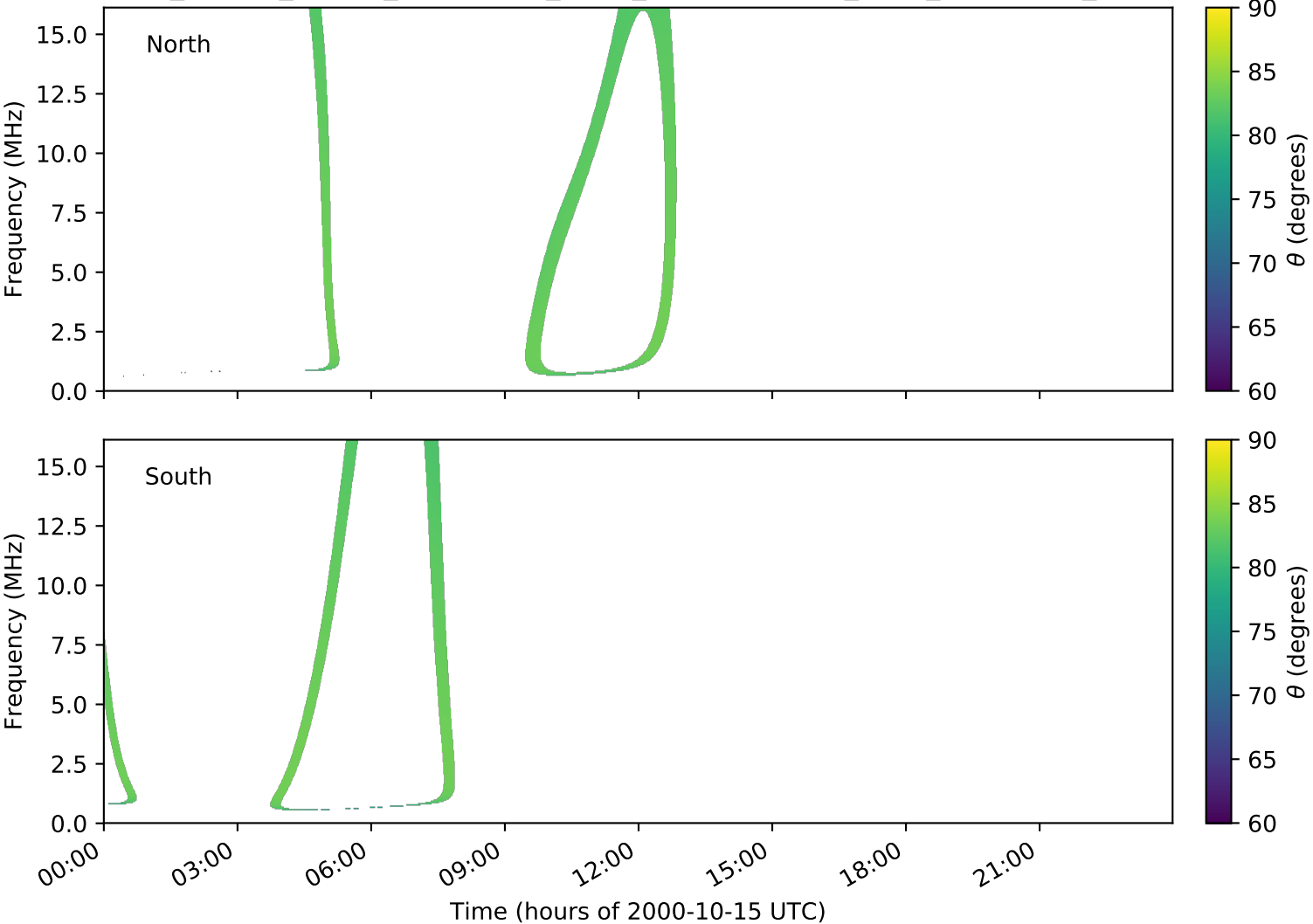
expres_cassini_jupiter_ganymede_isaac_lossc-wid1deg_3kev_20001015_v01.cdf
