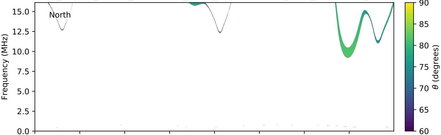
expres_cassini_jupiter_ganymede_isaac_lossc-wid1deg_3kev_20001014_v01.cdf
