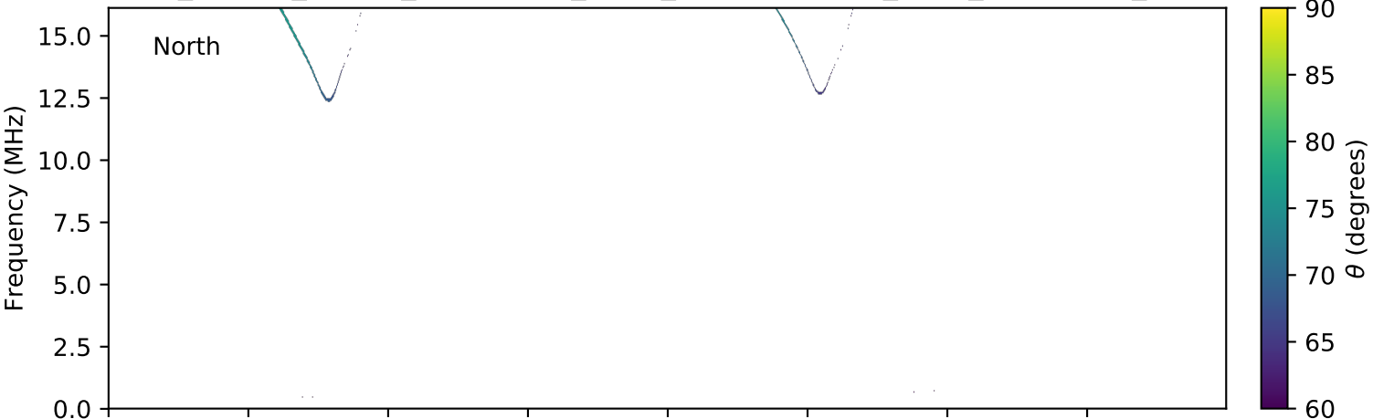
expres_cassini_jupiter_ganymede_isaac_lossc-wid1deg_3kev_20001013_v01.cdf
