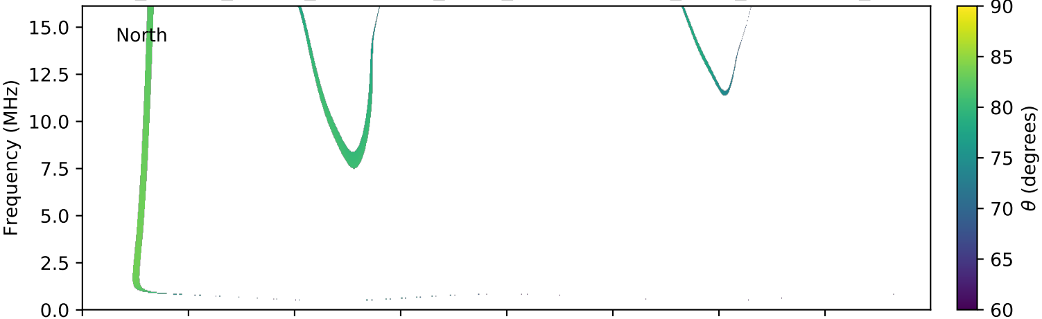
expres_cassini_jupiter_ganymede_isaac_lossc-wid1deg_3kev_20001012_v01.cdf
