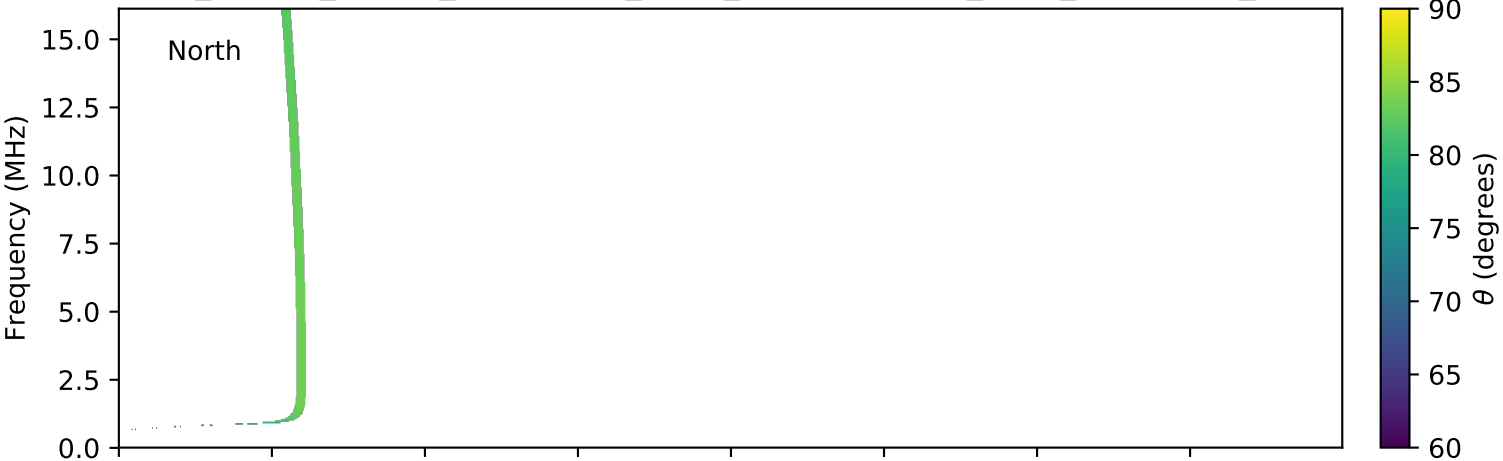
expres_cassini_jupiter_ganymede_isaac_lossc-wid1deg_3kev_20001008_v01.cdf
