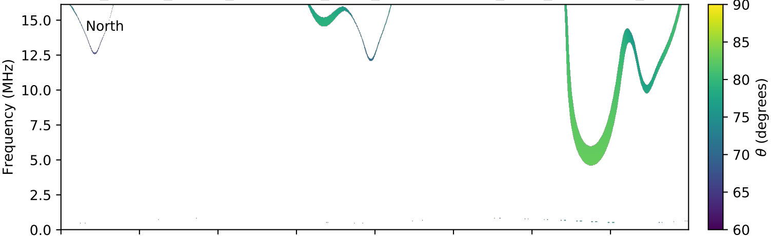
expres_cassini_jupiter_ganymede_isaac_lossc-wid1deg_3kev_20001007_v01.cdf
