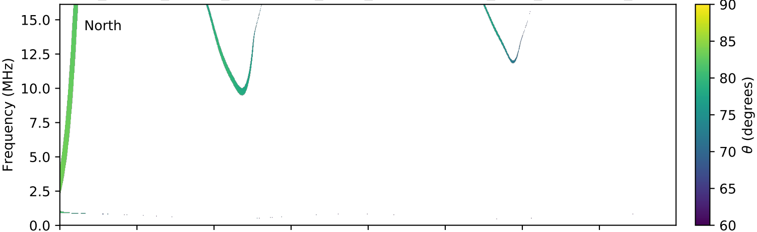
expres_cassini_jupiter_ganymede_isaac_lossc-wid1deg_3kev_20001005_v01.cdf
