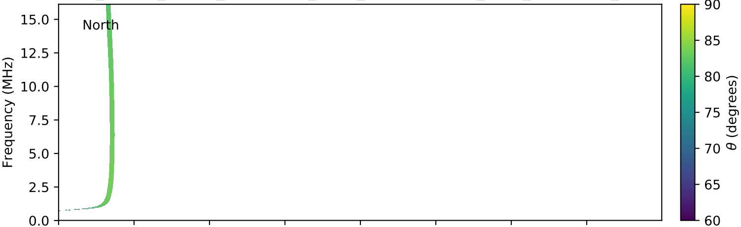
expres_cassini_jupiter_ganymede_isaac_lossc-wid1deg_3kev_20001001_v01.cdf
